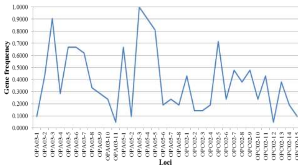
Fig. 2 Gene frequency for 34 loci based on RAPD marker analysis
