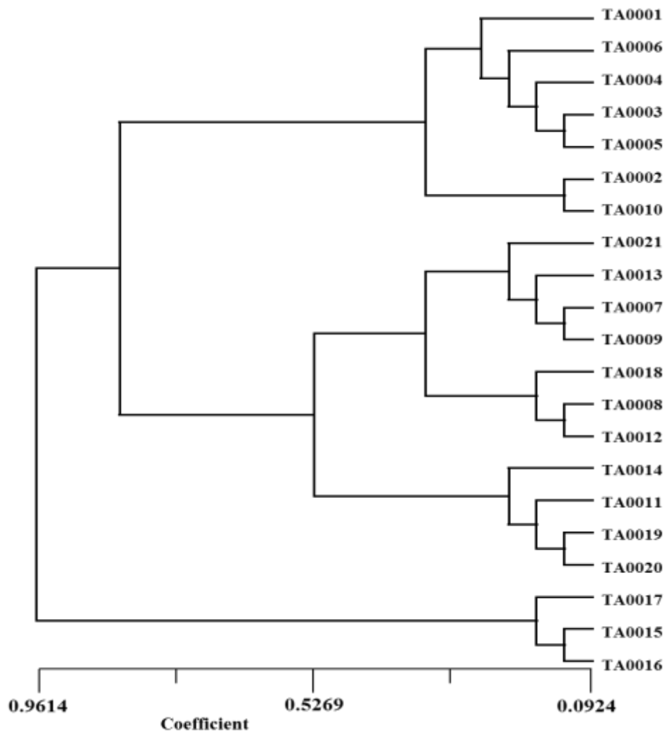
Figure 4. UPGMA dendrogram showing the relationship and diversity among 21 genotypes of T. anguina based on Nei's (1972) genetic distance.
